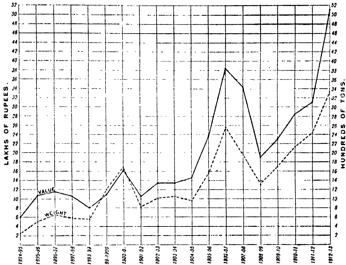
FIG. 6.—Exports of Indian mica during the past 20 years.
